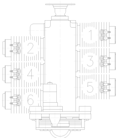
Figure 5 – 3300 Cylinder Denomination
