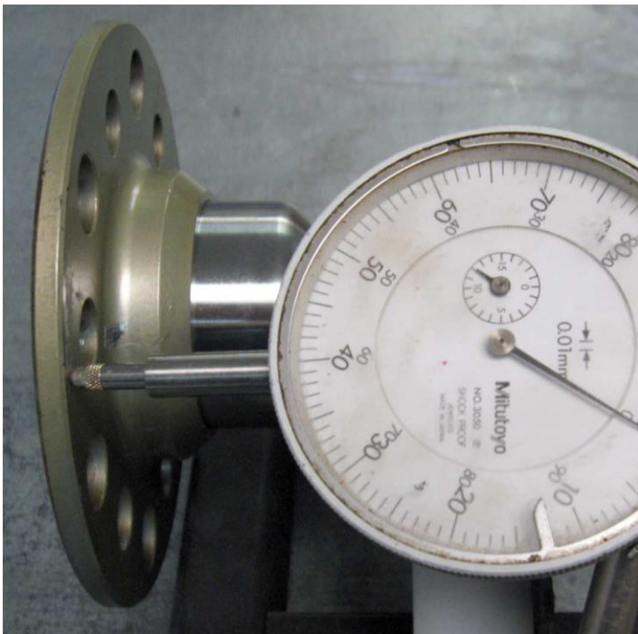
Figure 49 – Dial Indicator Position for Crankshaft & Prop Flange Run Out
