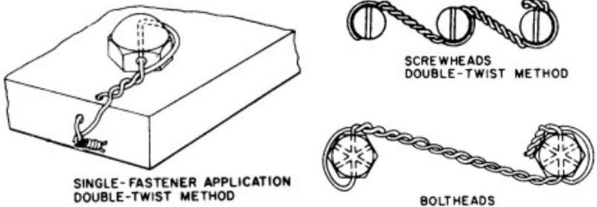
Figure 47 – Safety Wire Details
