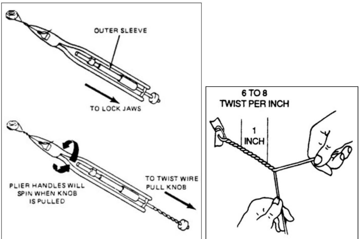
Figure 48 – Safety Wire Installation Using a Twister/Pliers & By Hand
