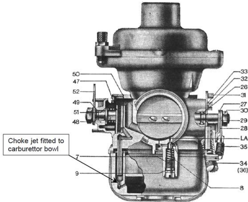
Figure 50 – Choke Schematic
